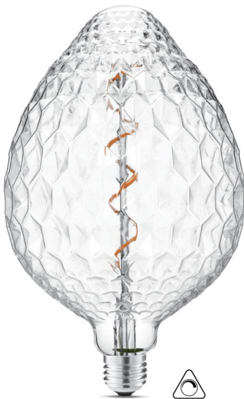
S150-Clear WATTAGE: 4.0W LUMEN: 240LM CCT: 2200K VOLATGE: 220-240V SIZE: 150X245MM
