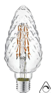
PC70-Clear WATTAGE: 4.0W LUMEN: 400LM CCT: 2700K VOLATGE: 220-240V SIZE: 70X160MM
