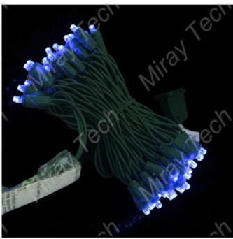
5mm LED Blue/Green Cord Model:MH2-70-5MM-B Cord: 22 AWG Voltage: 120V
