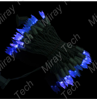
M5 LED Blue/Green Cord Model:MH1-70-M5-B Cord: 22 AWG Voltage: 120V
